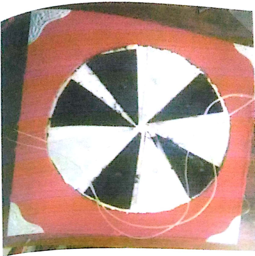
Designed Pyranometer without Glass
