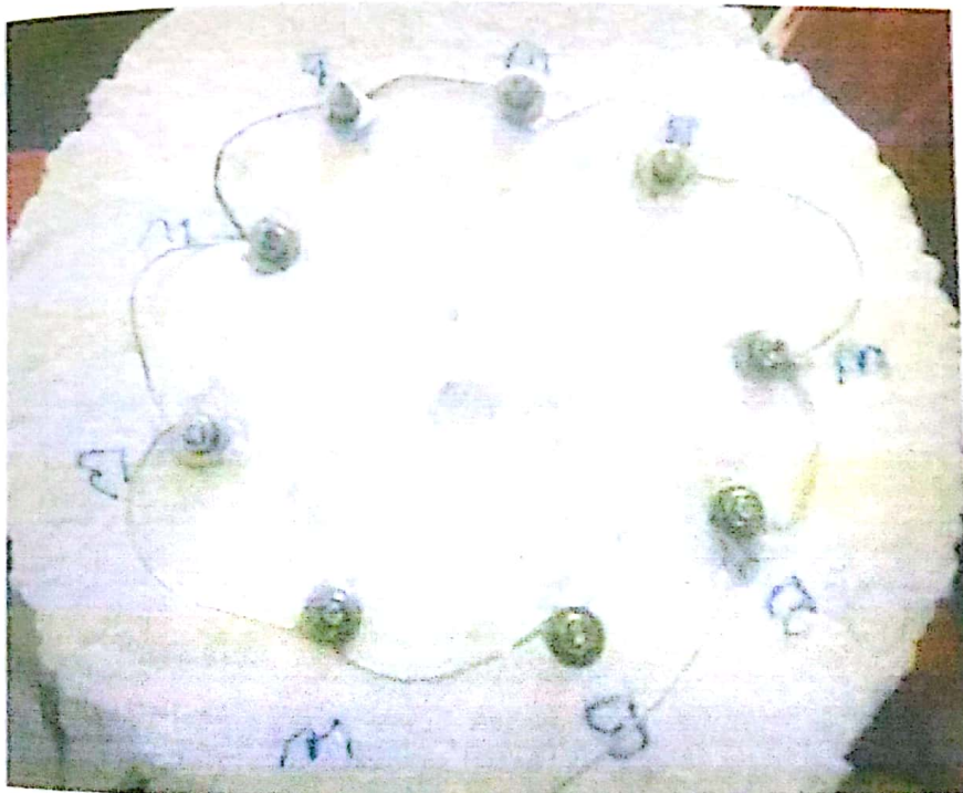
Internal layer of Designed Pyranometer
